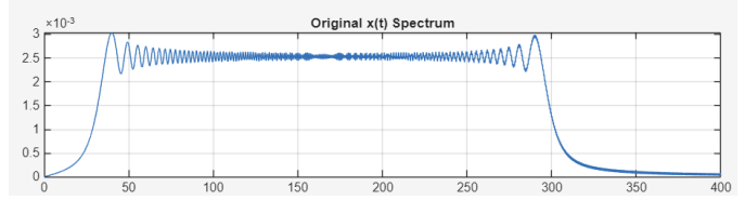
Figure 3. Magnitude Spectrum of the Original Signal x(t) .
