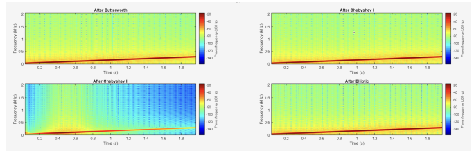
Figure 12. Spectrogram for Butterworth, Chebyshev I, Chebyshev II, and Elliptic Filters.
