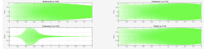
Figure 11. Comparative Time-Domain Waveforms for all Four Filter Topologies.
