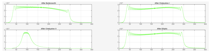
Figure 13. Frequency Sweep for Butterworth, Chebyshev I, Chebyshev II, and Elliptic Filters.
