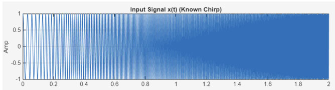
Figure 2. Input Signal x(t) (Known Chirp) in the Time-Domain.
