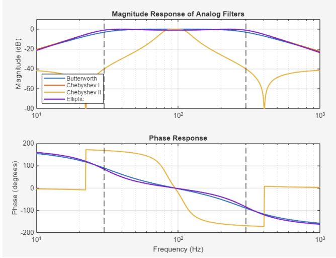
Figure 14. Bode Plot for Butterworth, Chebyshev I, Chebyshev II, and Elliptic Filters.
