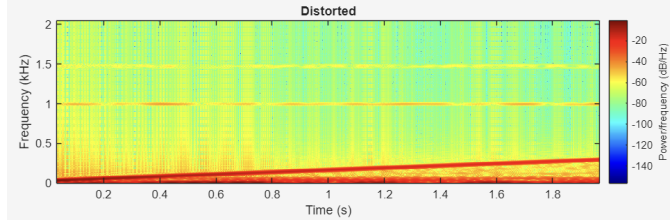
Figure 7. Distorted Signal y(t) Spectrogram Frequency Sweep.
